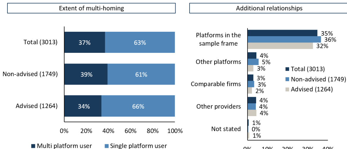
Figure 9: Multi-homing
